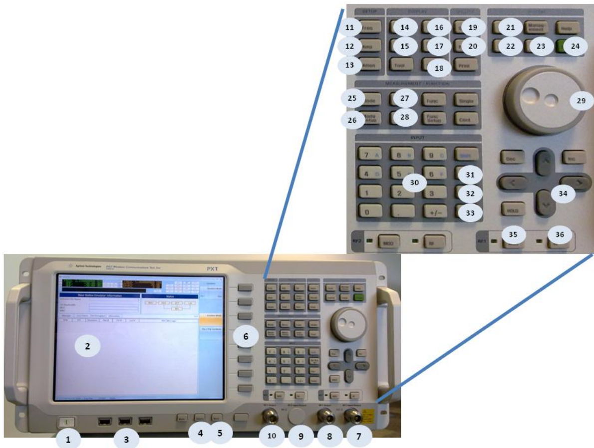
Figure 3-1 Front Panel
