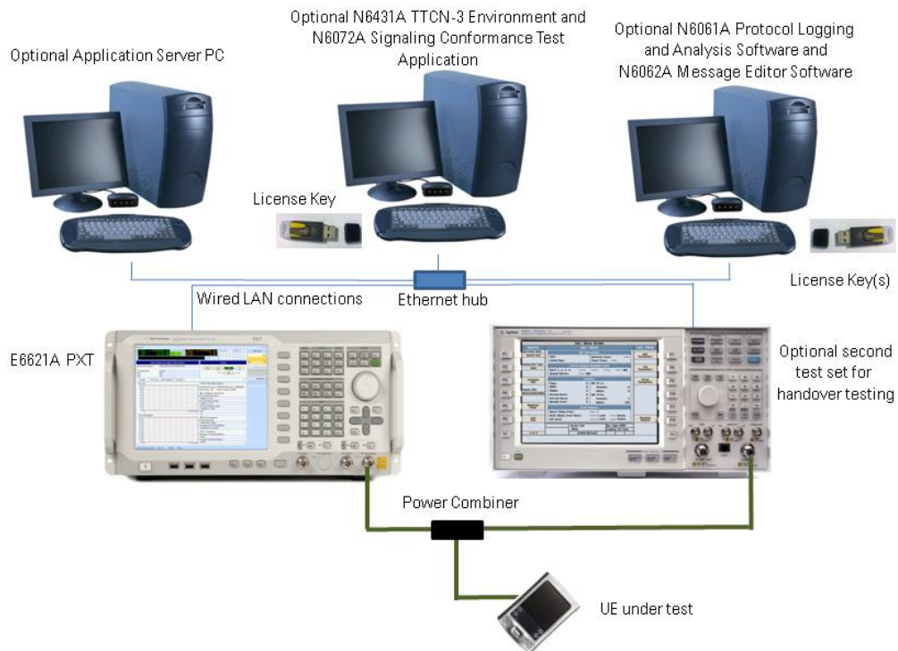
Figure 4-1: Example Test Setup
