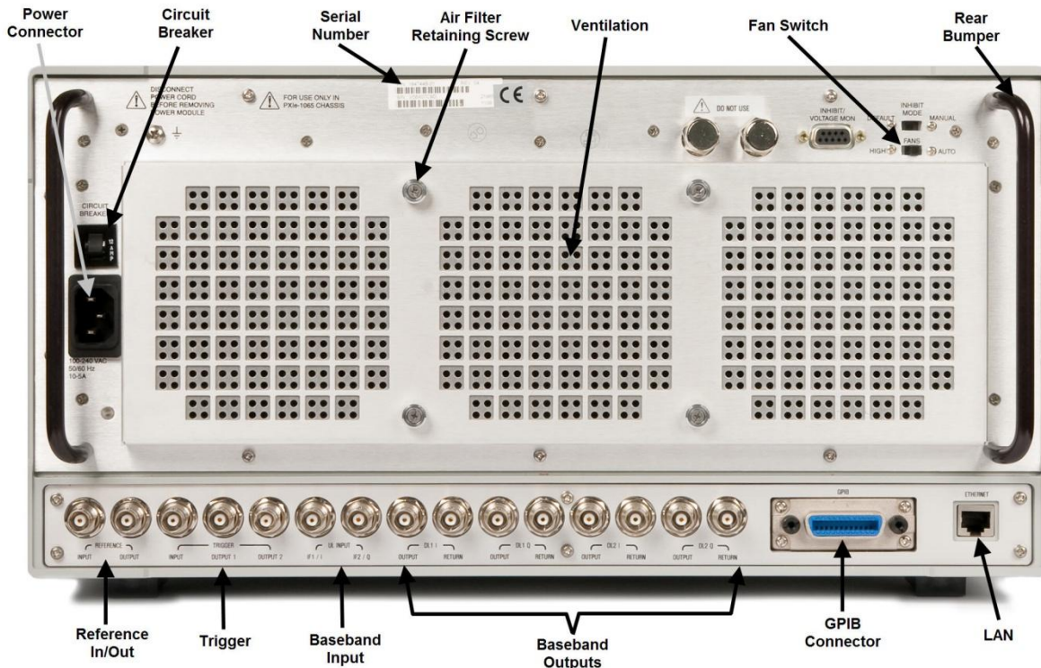
Figure 3-2 Rear Panel
